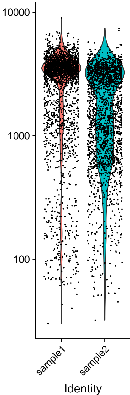
nFeature_RNA
