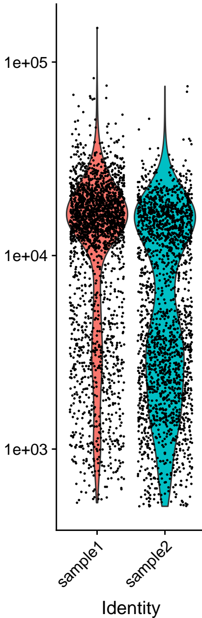
nCount_RNA
